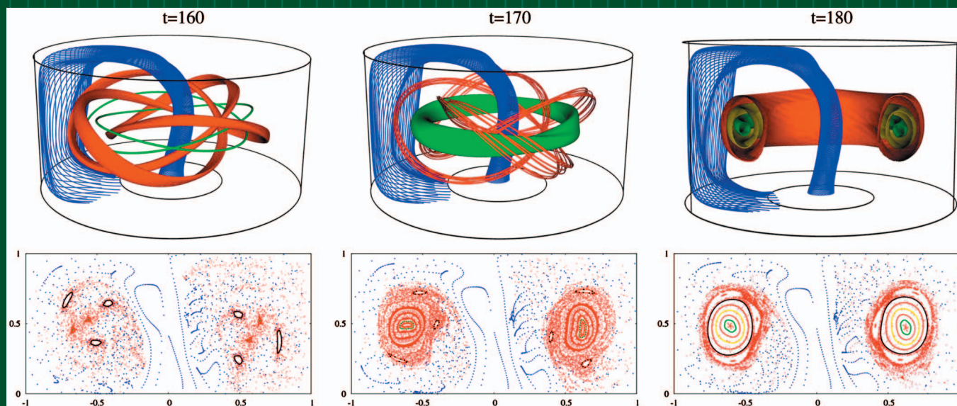
Relaxation of spheromak configurations with open flux by P. L. García-Martínez and R. Farengo
