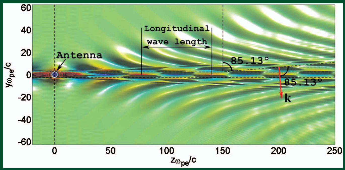
Generation of whistler waves by a rotating magnetic field source
